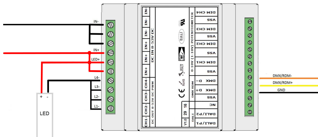
BUS DMX512/RDM WIRING DIAGRAM L406MA02T4A01 - FIGURE N. 4
