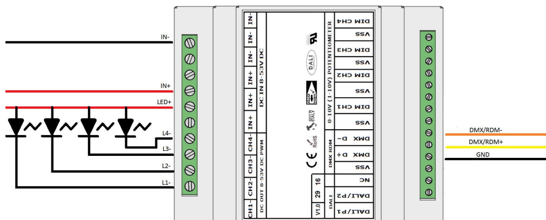
BUS DMX512/RDM WIRING DIAGRAM L406MA02T4A01 - FIGURE N. 3
