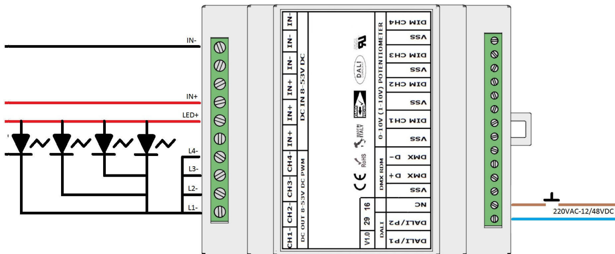
PUSH INTERFACE WIRING DIAGRAM L406MA02T4A01 - FIGURE N. 9
