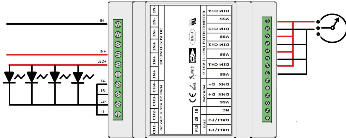
POTENTIOMETER WIRING DIAGRAM SINGLE CHANNEL L406MA02T4A01 - FIGURE N. 12
