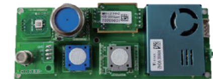
ZPHS01B 9-in-1 Air Quality Detection Module (CO 2 , PM2.5/10, TVOC, CO, O 3 , CH 2 O, NO 2 , T&H)
