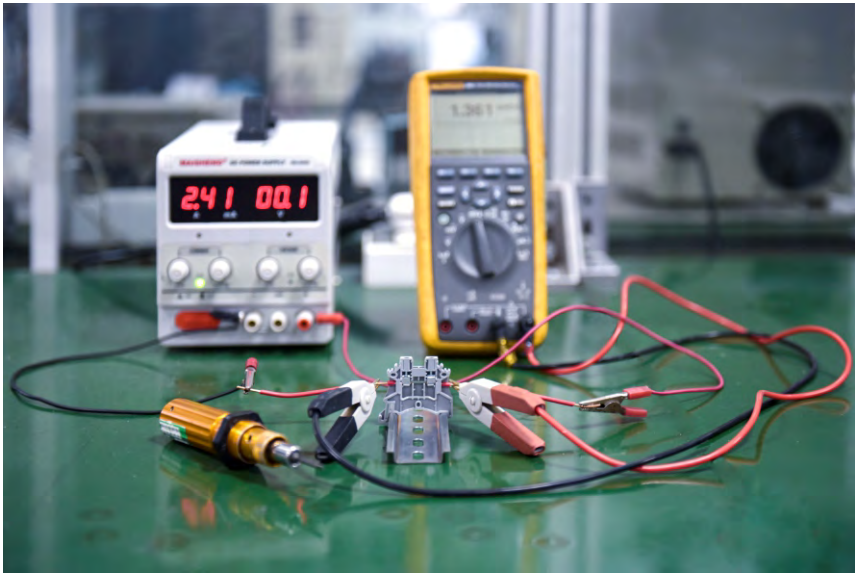
Din Rail Terminal Blocks Voltage-drop Test
