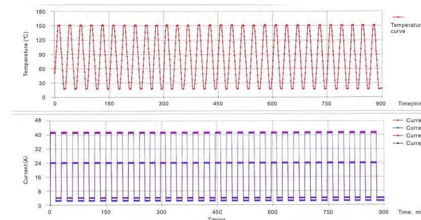
Aging Cycle Test
