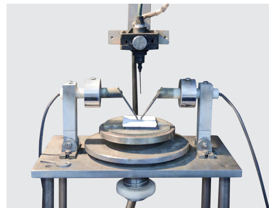
Din Rail Terminal Blocks Comparative Tracking Test
