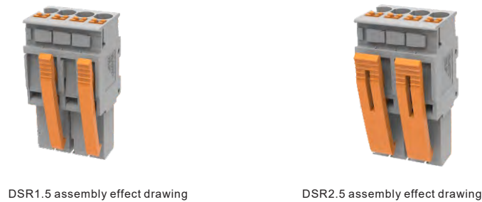
The self-assembled plug can be matched with DSR1.5/2.5 clip accessories,flexible field installation
