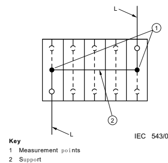
b) Group Temperature-rise test layout
